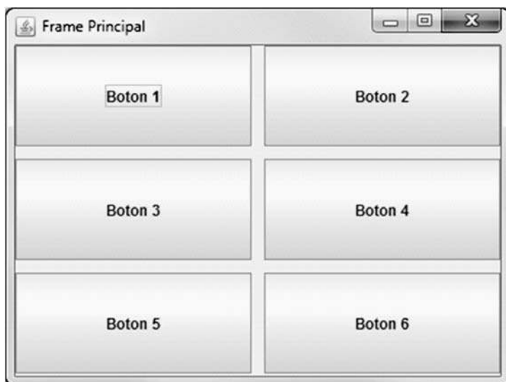
Figura 45. Grid Layout
