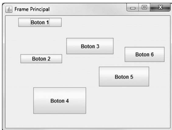
Figura 42. Absolute Layout
