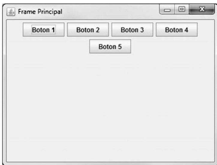
Figura 44. Flow Layout
