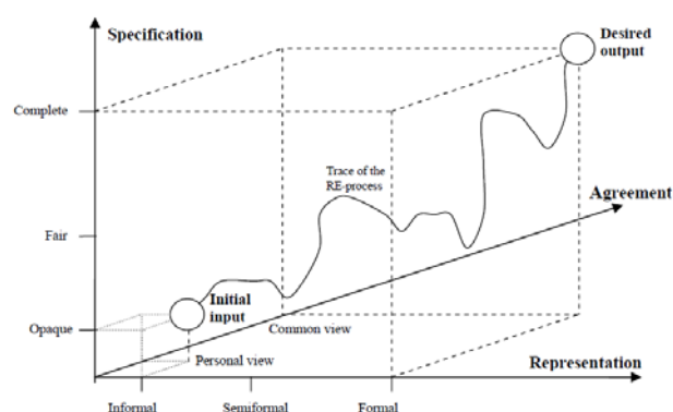
Figura 1. NATURE framework [26, 27]
