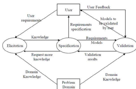
Figura 2. Iterative Requirements Engineering Process Model [28]
