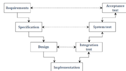
Figura 12. Model V [42]
